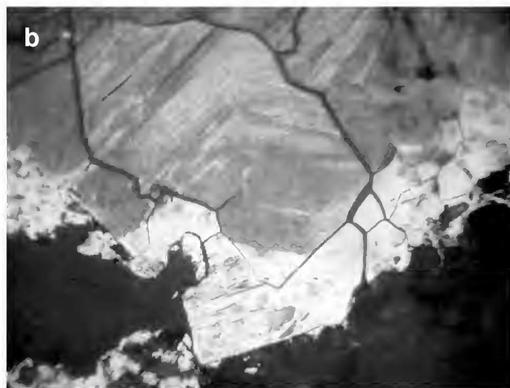
Fig.25- Reflected light photomicrographs: a) Polycrystalline troilite indicative of strongly shock with two bronzite crystals (dark gray) inclusions; b) - Polycrystalline and twinned troilite indicative of strongly shock. Length of field 0.2mm.
